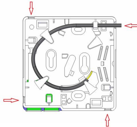
Entry ports
