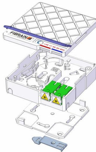
Outlet design
