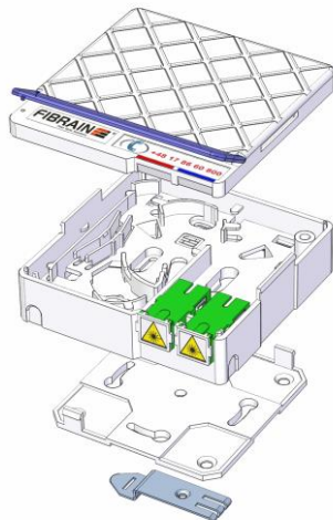
Outlet design
